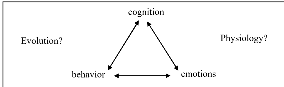
Figure 1.1: Cognitive Triangle
